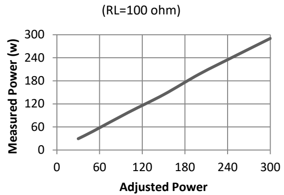
Bipolar Ablation (RL=100 ohm)
