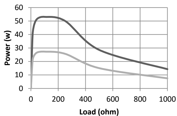
Auto Bipolar Coag.
