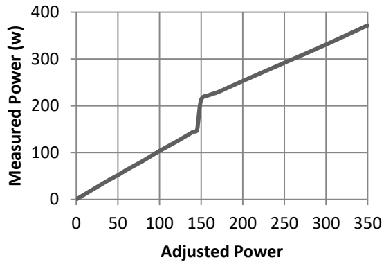
Bipolar Resection (RL=50 ohm)
