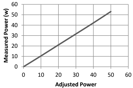
Auto Bipolar coag. (RL=100 ohm)
